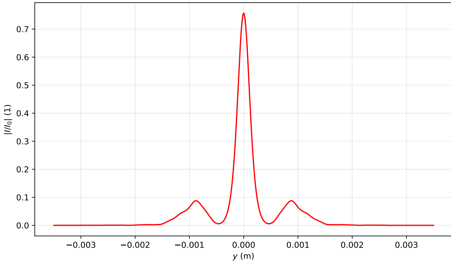
Intensity profile I(x=0, y, z=2.149)/I_0 , P_{in}=8.5P_{cr} , artificial time
